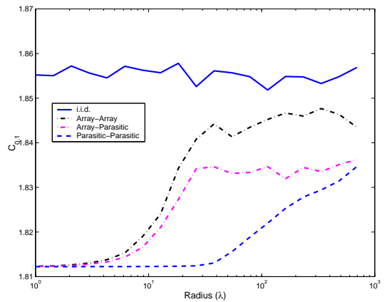
Figure 8: The channel capacity at 10% outage versus the radius of the scattering disc. Only N=M=2 of the 4 modes in the parasitic antenna in Figure 2 are used. SNR=4 dB.
